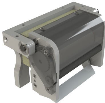
Fig. 3: Render of the dribbler
