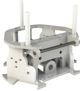
Fig. 5: Render of the frame
