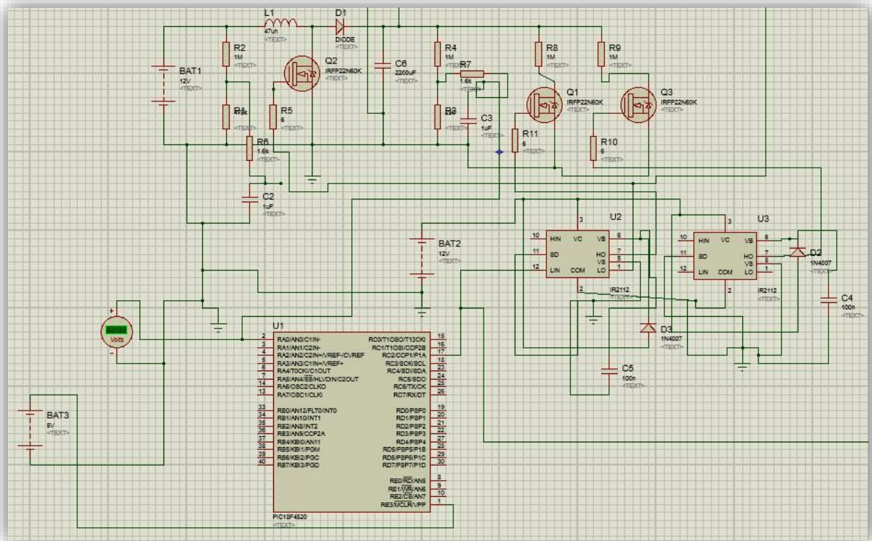
Figure 3: Kicker Simulation Schematic Diagram
