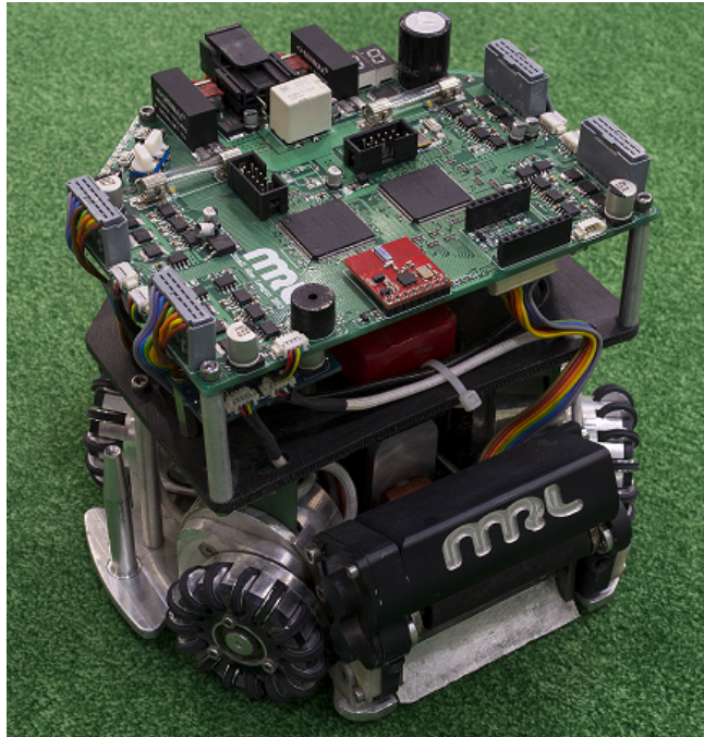
Fig. 1. MRL robot for 2015 competitions
