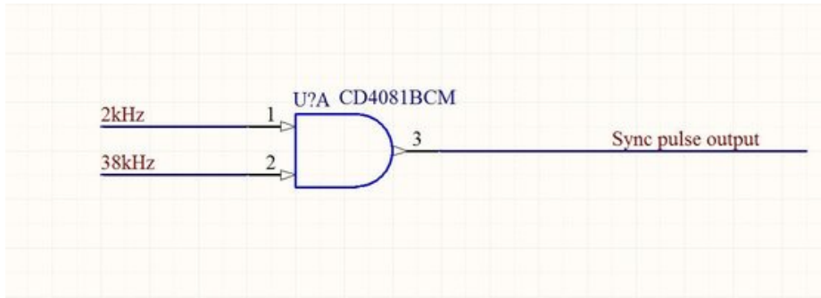
Fig. 11. data syncing with and gate
