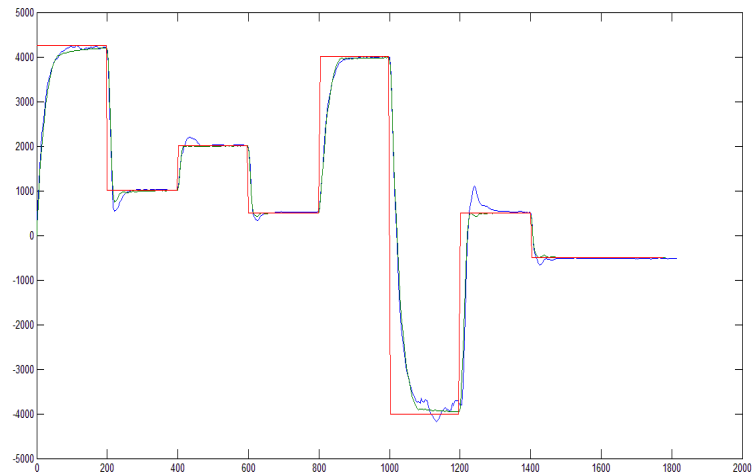
Figure 12 PID controller vs PD core controller with CTS
