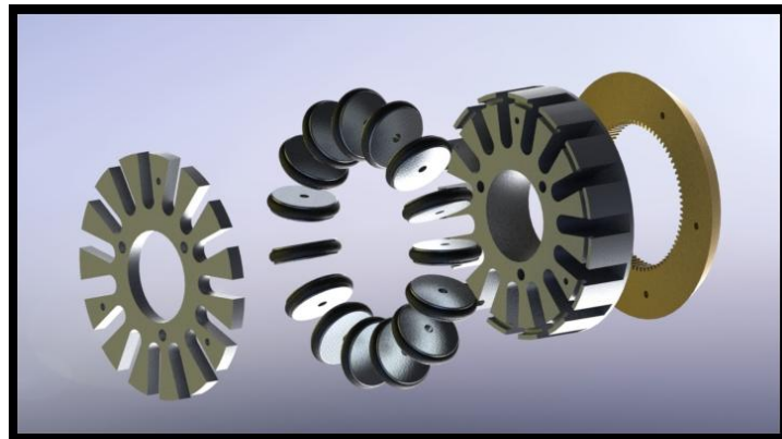
Figure 8 3D figure of the robot wheel
