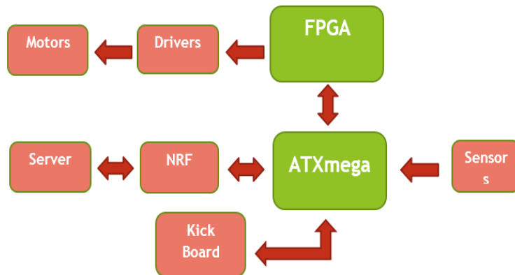
Figure 2 block diagram of the electrical system.
