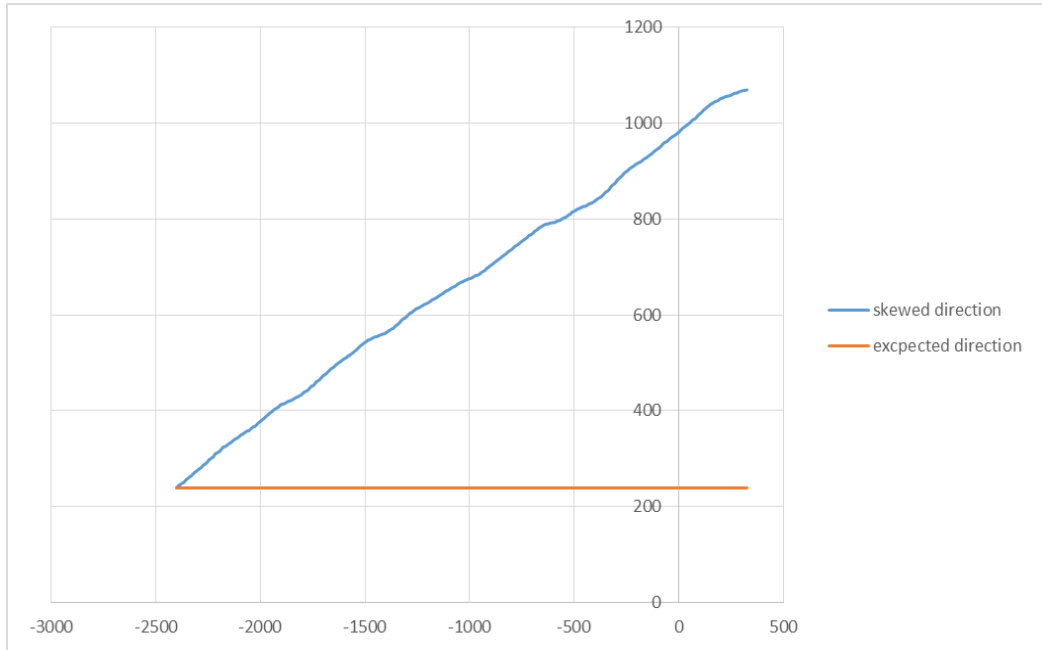
Figure 13 Diversion in direction of displacement
