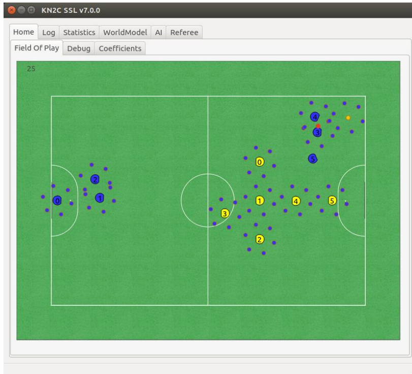
Figure 11 Output of A* Algorithm
