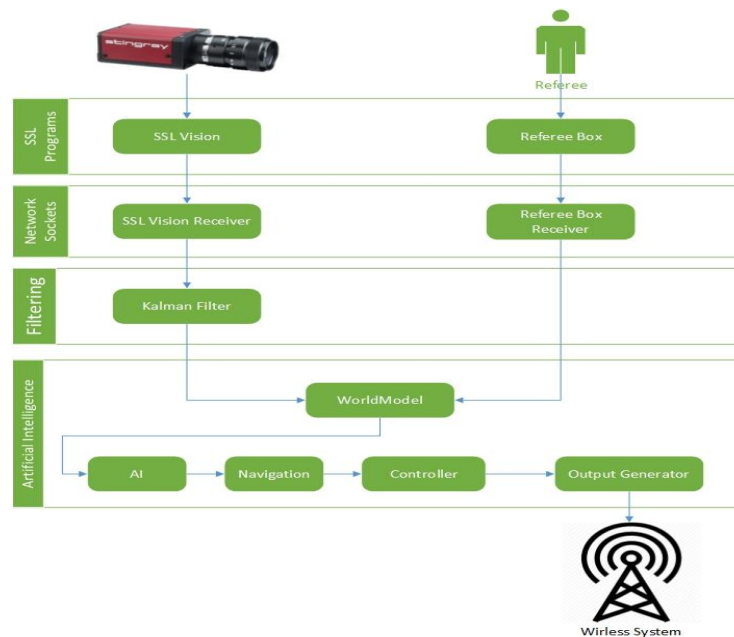
Figure 10 Overview of Software System
