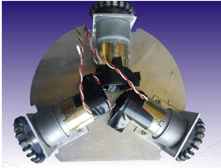
Figure 5. Mechanical design
