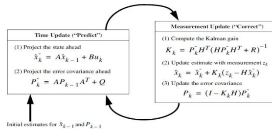
Figure 9. A complete picture of the operation of the Kalman filter
