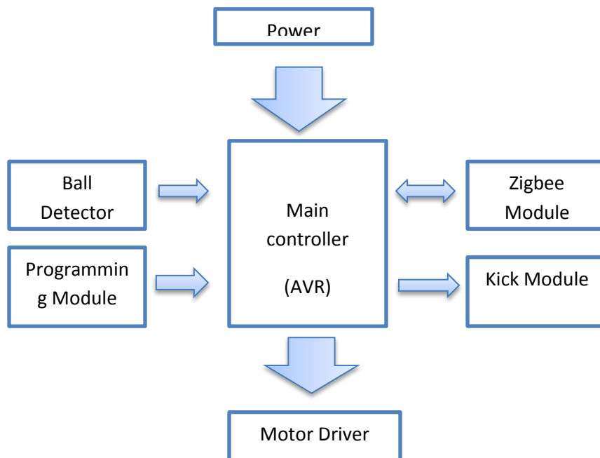
Figure 2. The electrical system's diagram
