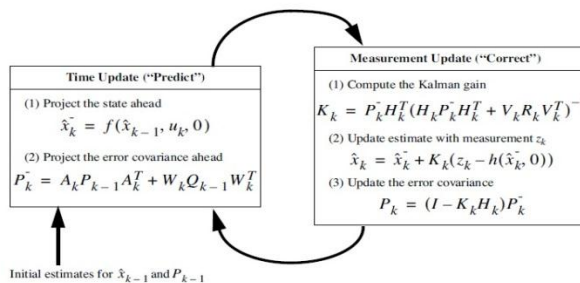
Figure 10. A complete picture of the operation of the extended Kalman filter
