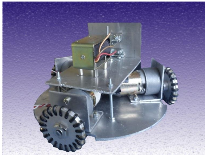
Figure 7. Magnetic kick system
