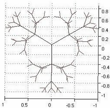
3D Fractals
